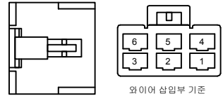
KET / 250 6F Housing Housing : MG610049 (White) To : Integral Unit
