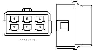
KET / 250 6M Housing Housing : MG620048 (White) To : Terminal
